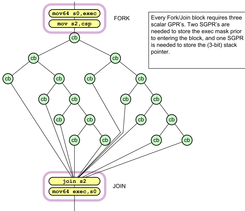
Figure 4. Example of Complex Control Flow Graph
