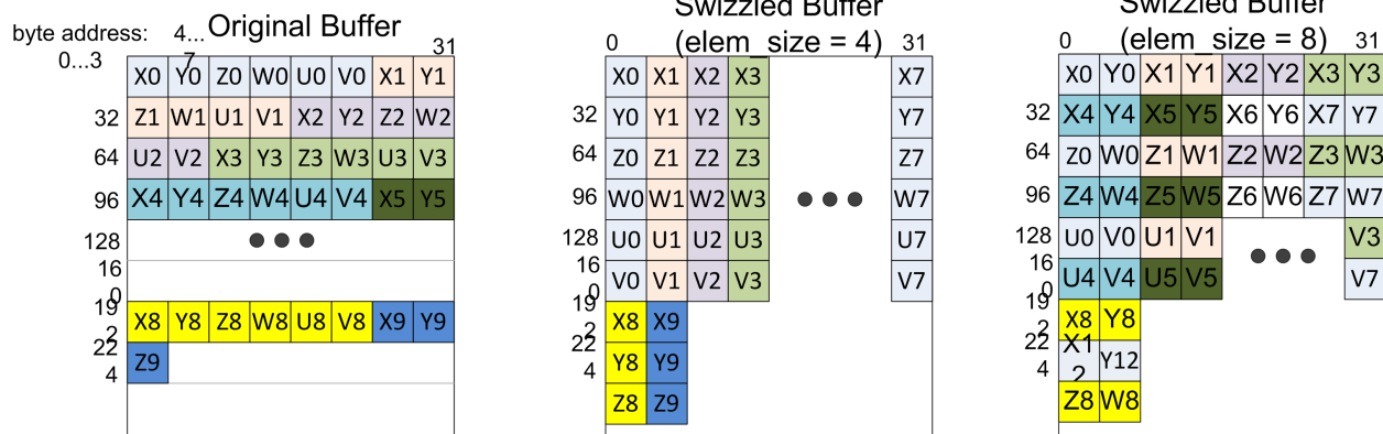
Figure 6. Example of Buffer Swizzling
