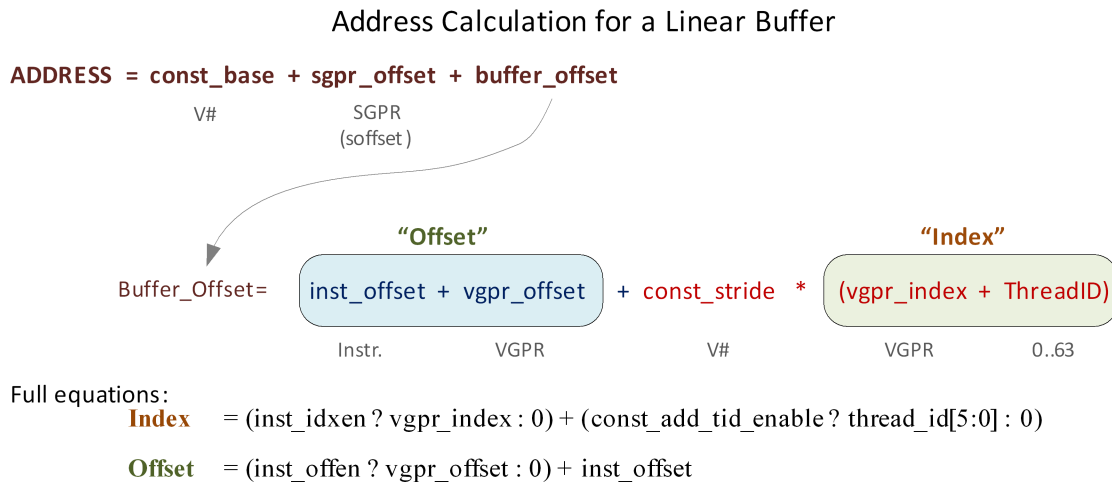
Figure 5. Address Calculation for a Linear Buffer
