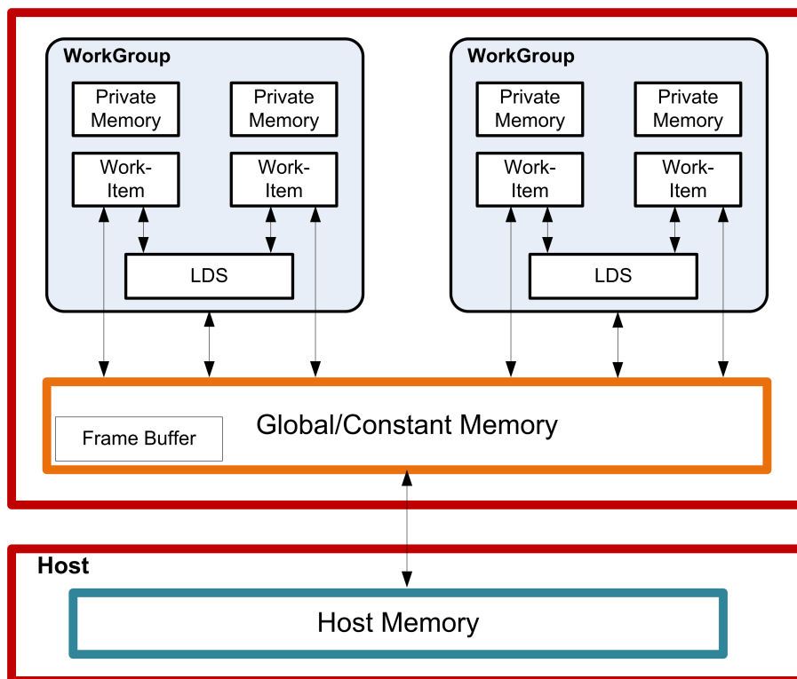
Figure 7. High-Level Memory Configuration
