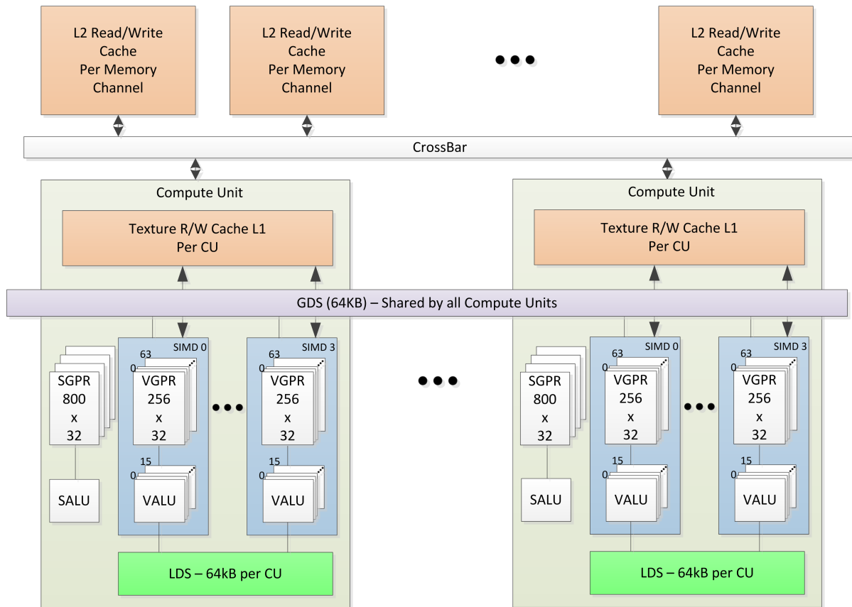
Figure 3. Shared Memory Hierarchy
